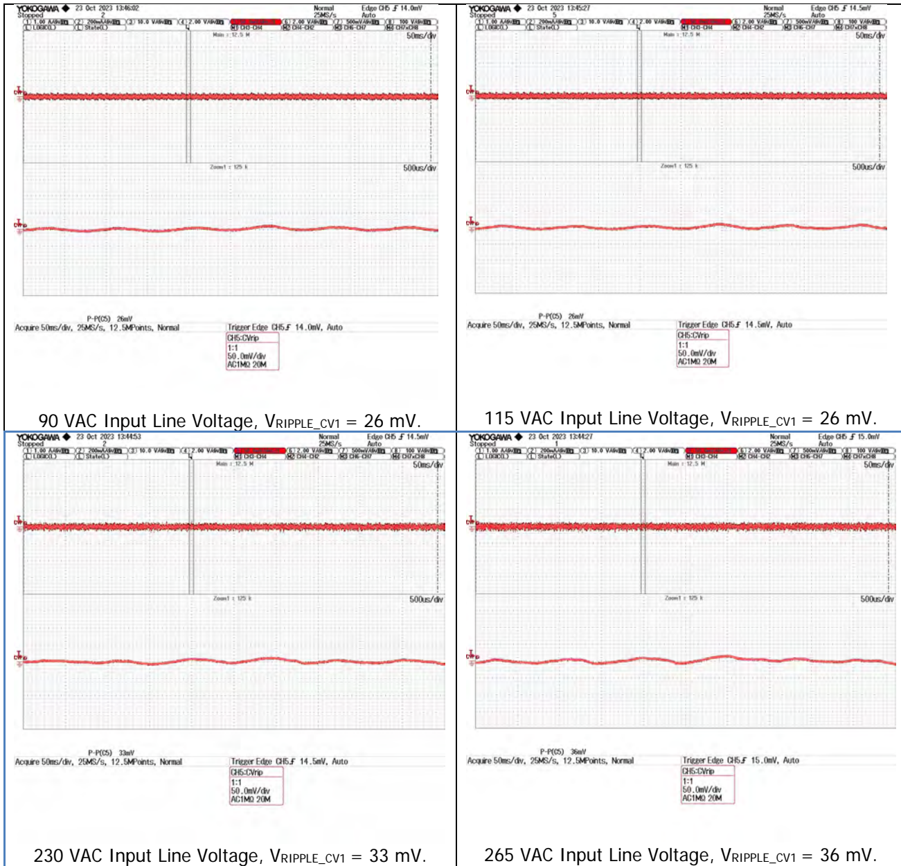
Figure 54 – VCV1 Ripple and Noise, LED = 29 V @ 400 mA.
