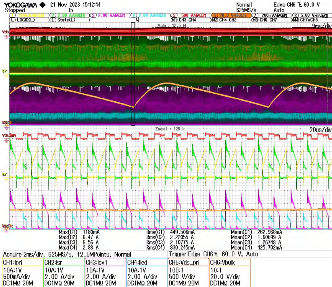
Figure 36 – Transformer All Winding Currents Over a Mains Cycle, 90 VAC.
