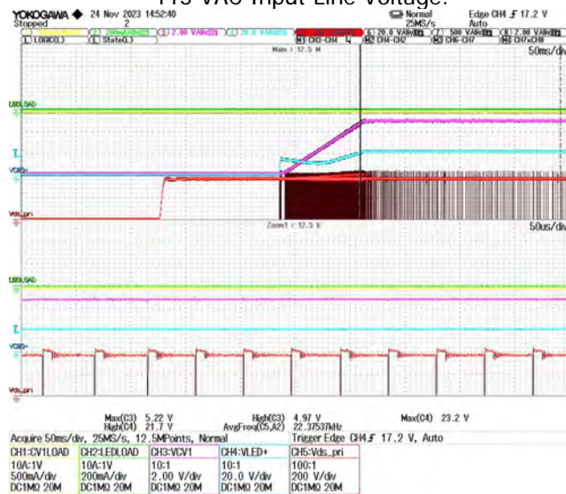
115 VAC Input Line Voltage.
