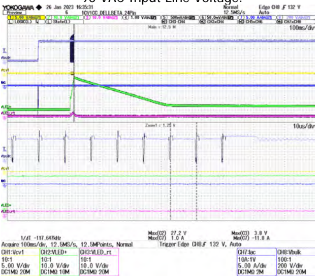
230 VAC Input Line Voltage.
