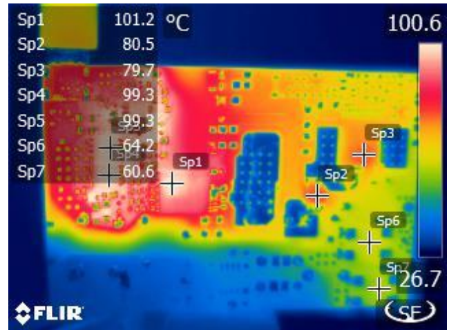
Figure 54 – Bottom Side. 265 VAC, Full Load.
